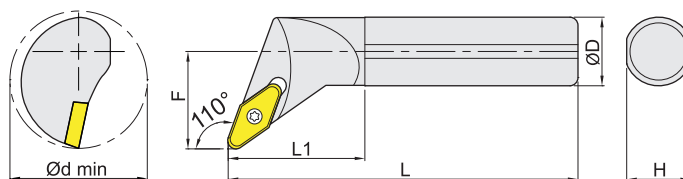
Steel shank (Right-hand shown) 鋼柄 右向示意圖
